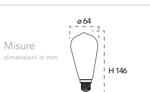
Lampadina a Led 4W, 240V
