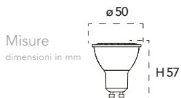
Lampadina a Led 6W, 240V
