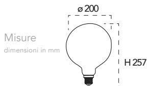
Lampadina a Led 8W, 240V
