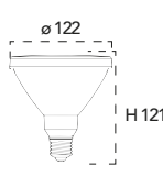
Lampadina a Led 18W, 240V
