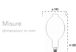
Lampadina a Led 8W, 240V
