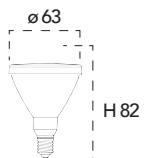
Lampadina a Led 8W, 240V
