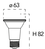
Lampadina a Led 7W, 240V
