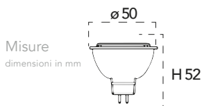
Lampadina a Led 6W, 12V AC/DC
