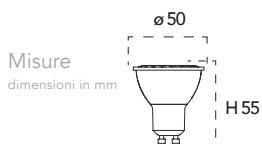
Lampadina a Led 9W, 240V
